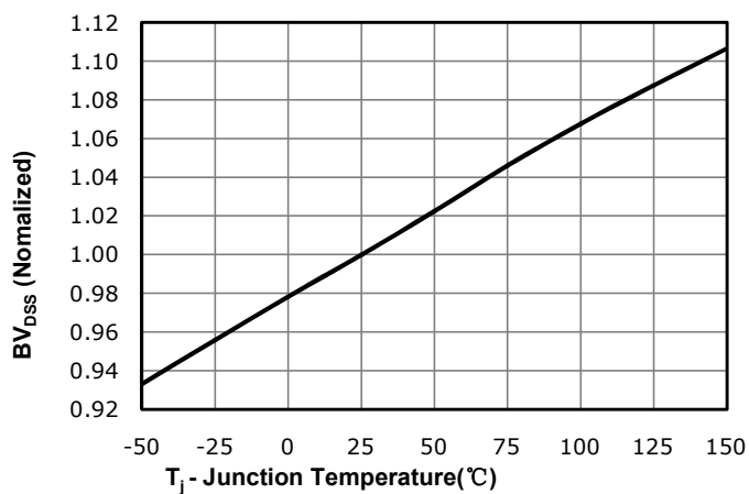
Fig 7: BV_{DSS} vs. Temperature
