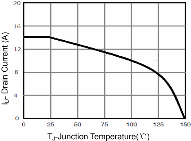
Figure 10 Current De-rating
