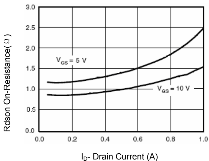
Figure 5 Drain-Source On-Resistance
